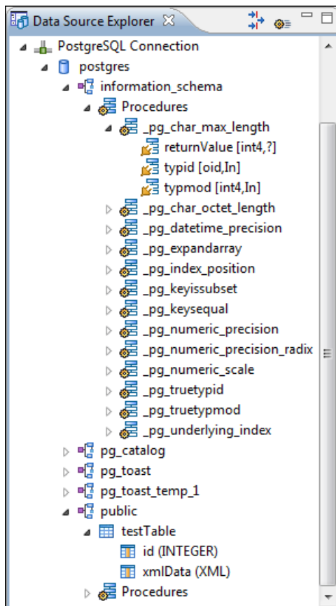
Figure 283: Browsing a PostgreSQL repository
