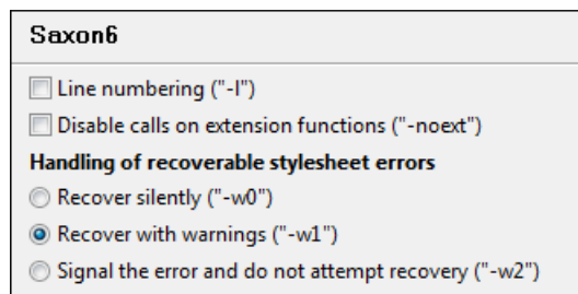
Figure 310: The Saxon 6 XSLT Preferences Panel
