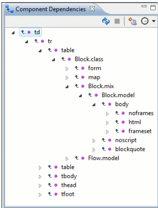
Figure 79: Component Dependencies View - Hierarchy for xhtml.rng
