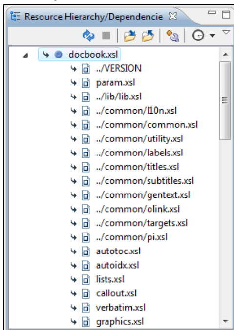
Figure 104: Resource Hierarchy/Dependencies View - Hierarchy for docbook.xsl
