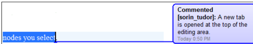
Figure 149: Comment Callouts
