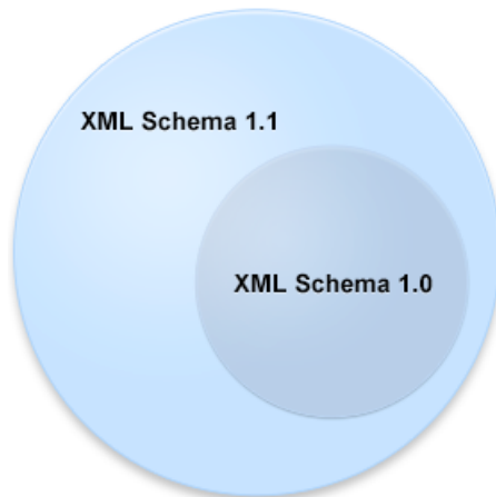
Figure 73: XML Schema 1.1
