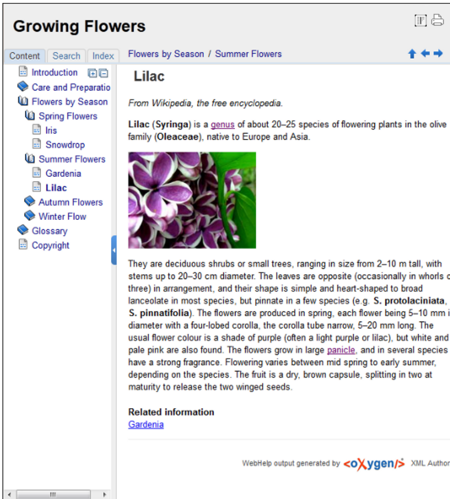
Figure 181: WebHelp Output
