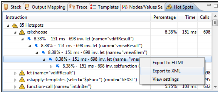
Figure 260: Hotspots View
