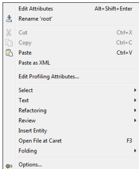
Figure 137: Contextual menu
