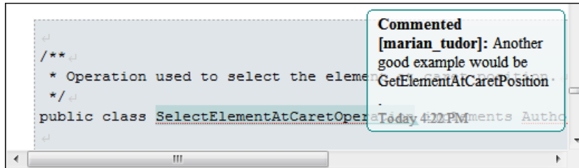
Figure 153: Transparent Callout
