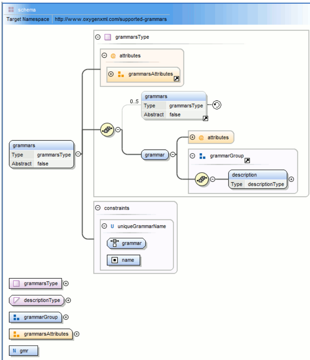
Figure 43: XML Schema Diagram
