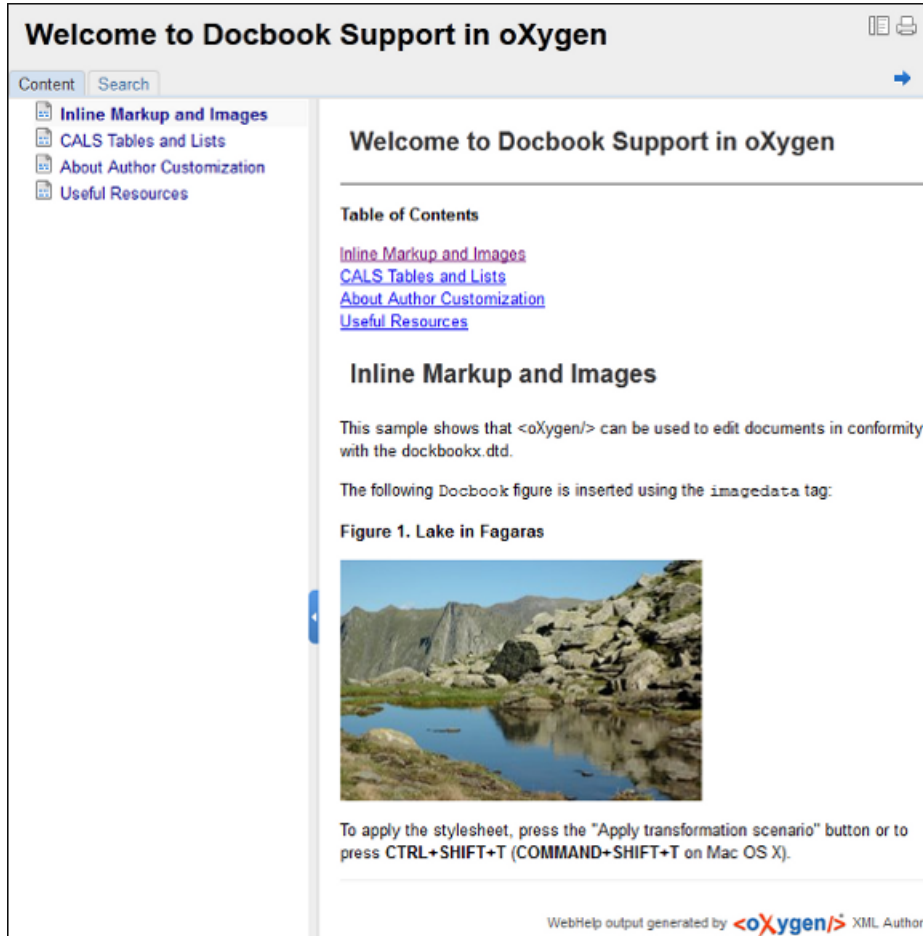
Figure 173: DocBook WebHelp
