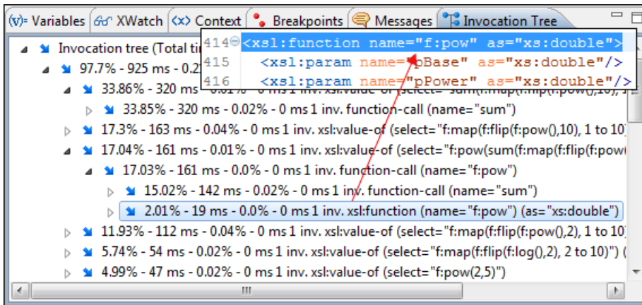
Figure 261: Source backmapping
